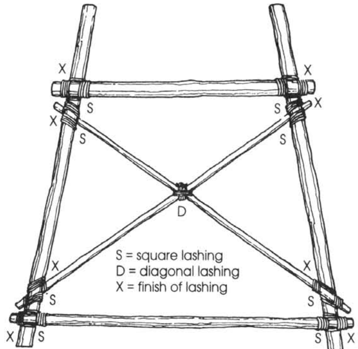
Lashings — front view
