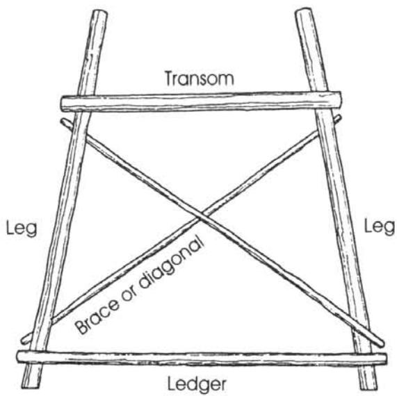
Layout of spars for square trestle — front view
