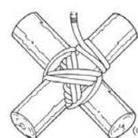
Diagonal lashing
