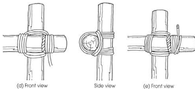
Square lashing
